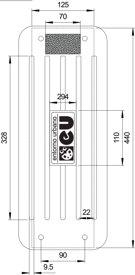
Upper side
