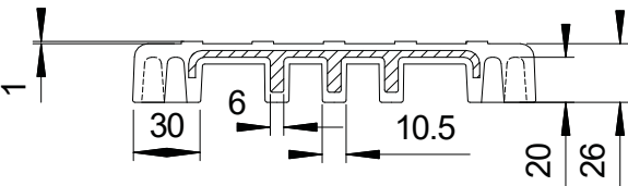
Cross section A-A'
